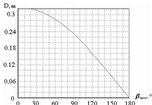
Fig. 3 – Dependence of diameter of torch of dispersion on spray corner
