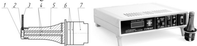
Fig. 7 – Ultrasonic atomizers of high-viscosity liquids
