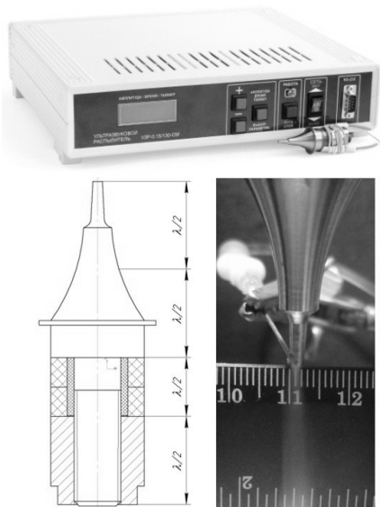
Fig. 5 – The appearance of the high-frequency atomizers
