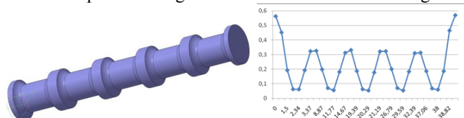
Fig. 3. The dependence of resonance frequency in the working tool on the number of lengths of half-waves (half-wave waveguides)
