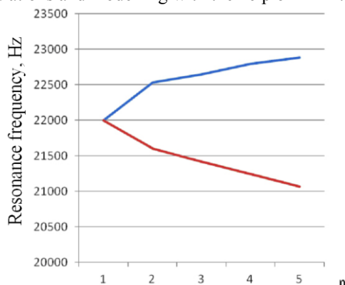
Fig. 3. The dependence of resonance frequency in the working tool on the number of lengths of half-waves (half-wave waveguides)
