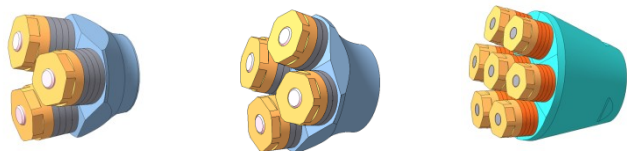
Fig. 7. The principal view of the piezoelectric transducers of increased power
