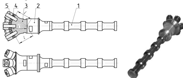
1 – the active working tool with the enlarged surface of the radiation, 2 – matching acoustic transformer (the concentrator), 3 – the working frequency reducing cover plate, 4 – the piezoelectric elements, 5 – reflective frequency reducing cover plates
