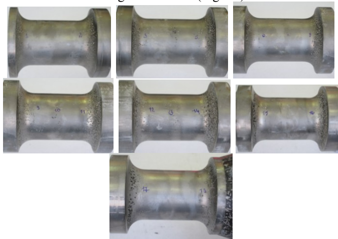
Fig. 12 – The cavitation wear of the working tool
