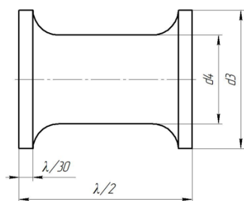
Fig. 1. The half-wave element of the waveguide
