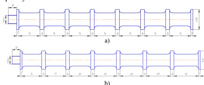
Fig. 4. The multiunit radiators for 22.9 and 22 kHz
