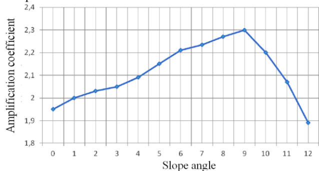
Fig. 9. The dependence of the amplification coefficient of the transducer on the slope angle of the plane
