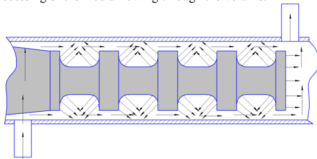
Fig. 11. The ultrasonic vibrating system in the running technological volume
